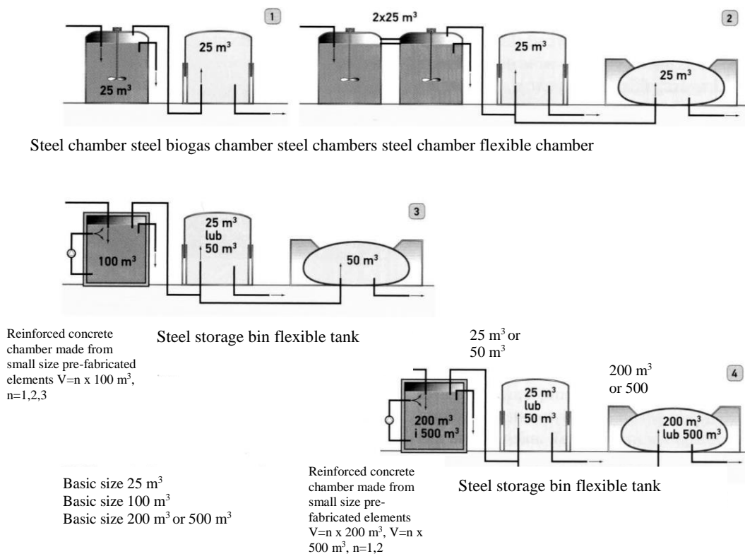
Fig. 3. Schematic diagrams of biogas systems with the fermentation chamber with a volume from 25 \text{ m}^3 to 500 \text{ m}^3 (and its multiple). Source: [4]
