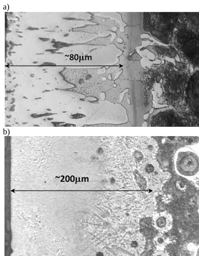
Fig. 3. The microstructure of the boronized zone by diffusion (a) and laser (b) treatment. Etched with nitride acid solution
