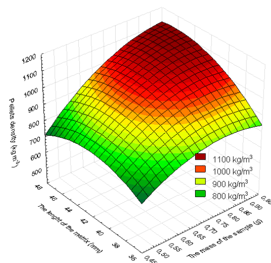
Fig. 4. Influence of material and process factors on the density of pellets obtained during the densification of a mixture of tobacco waste and potato pulp in an open chamber: a) influence of pulp content and process temperature, b) influence of mass of the densified sample and length of matrix openings
