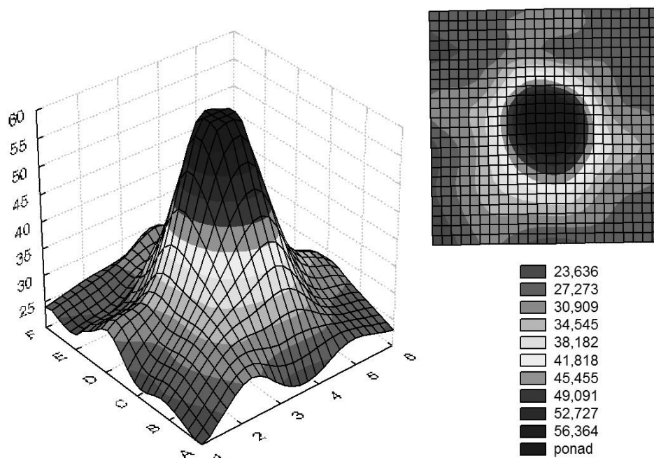
Fig. 1. Temperature distribution on the floor (°C) in piglets' nest with the use of the traditional infra-red lamp [11]
