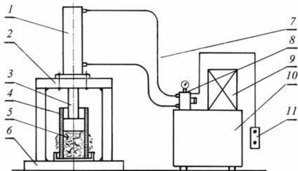
Fig. 1. Test stand diagramme: 1 – cylinder, 2 – frame, 3 – piston, 4 – basket press, 5 – raw material, 6 – base, 7 – conduit, 8 – servo valve with a packing gland, 9 – motor, 10 – container, 11 – guide-pin
