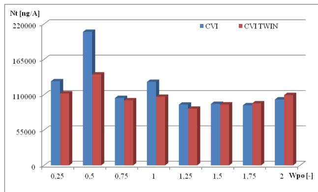
Fig. 7. The total deposition of spray liquid
