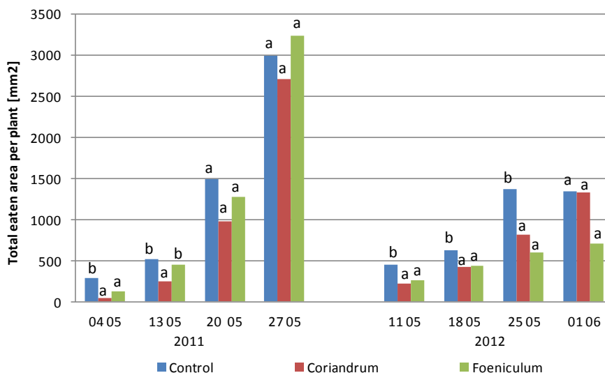
Fig. 2. Total eaten area per plant (mm 2 ) caused by Sitona spp. adult depending on cultivation method. Mean followed by the same letter in a given date respectively are not significantly different at p < 0.05 , factor: cultivation method. For treatments explanation see fig. 1
